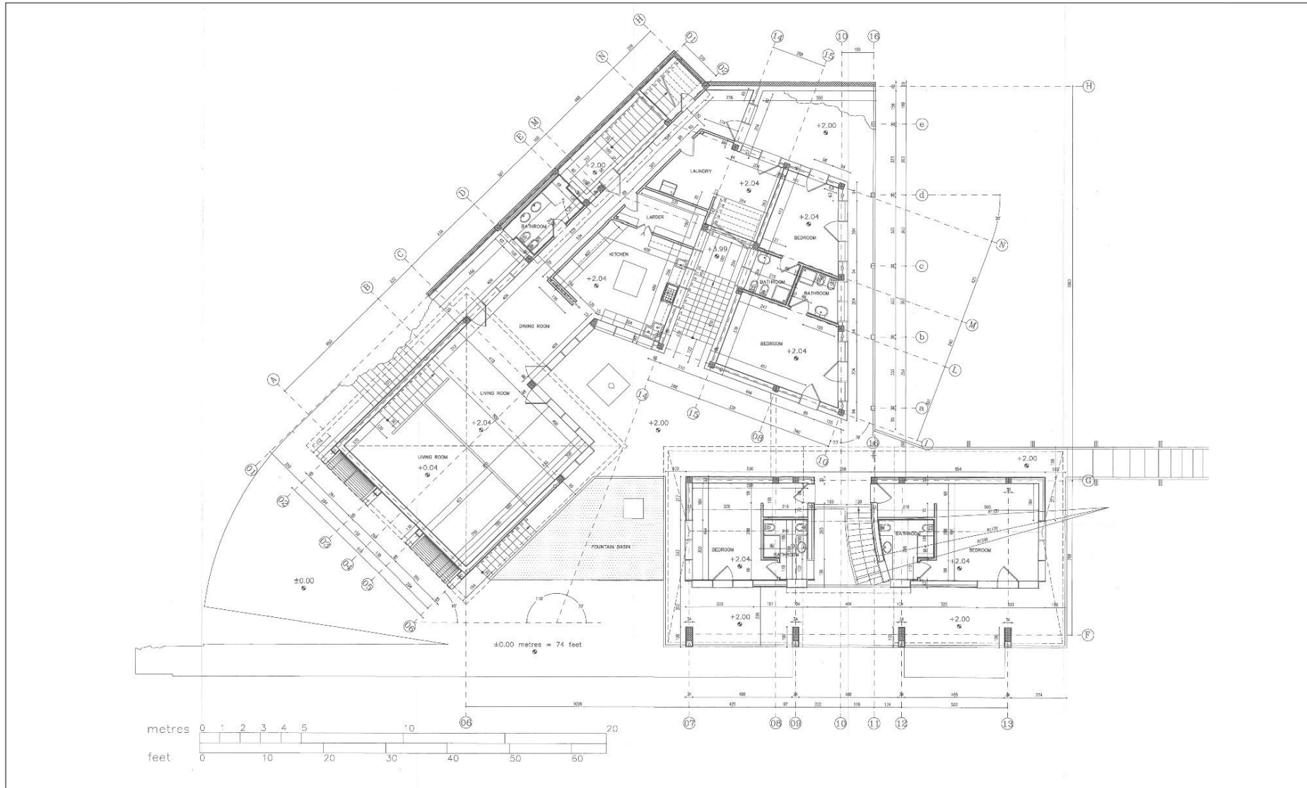
FLOOR PLAN 1
