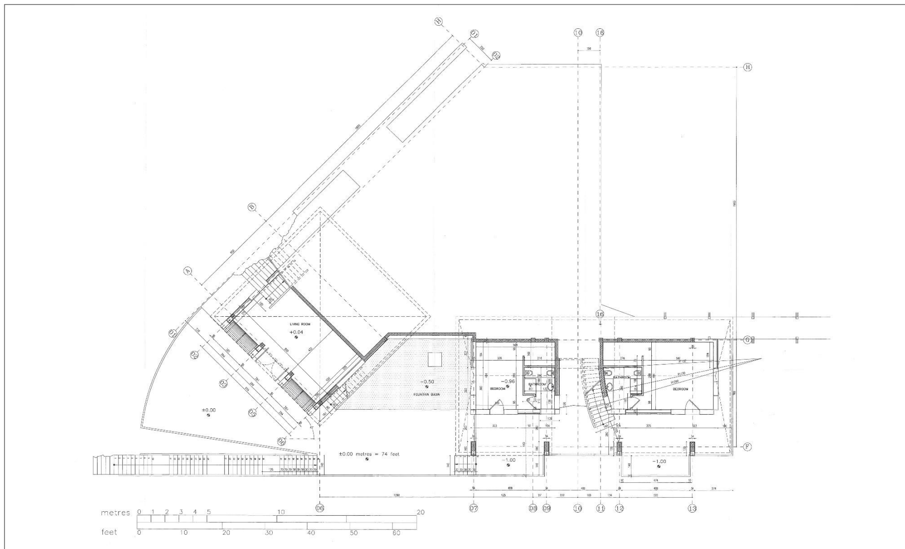
FLOOR PLAN 2
